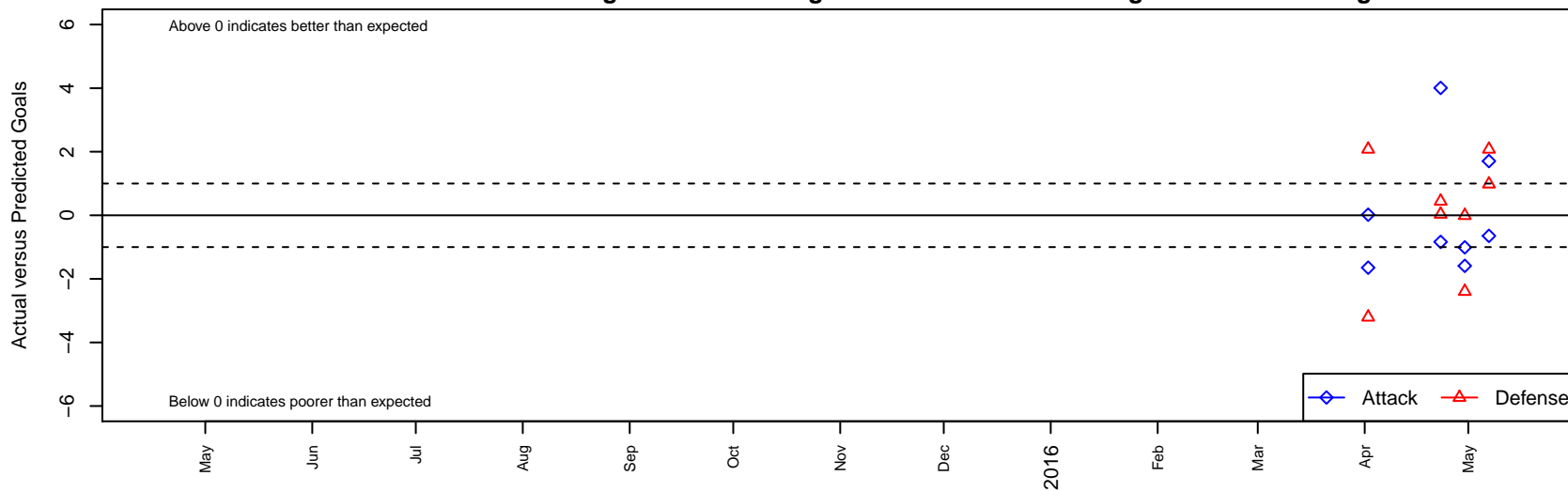
Union Couny United G03 Dots are actual minus expected GF (blue circles) and GA (red triangles). Blue line is smoothed change in attack strength. Red is smoothed change in defense strength.
